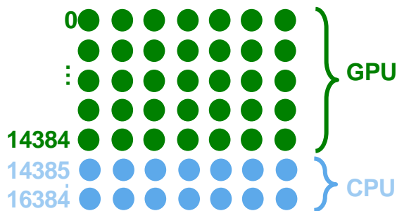
Figure 3: Work distribution between CPU and GPU
