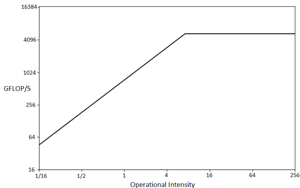
Figure 6: Performance roofline for a NVIDIA Pascal P100 GPU. Peak double precision floating point performance are 5.3 TFlop/s. The peak sustainable memory bandwidth (to device memory) is 732 GB/s.
